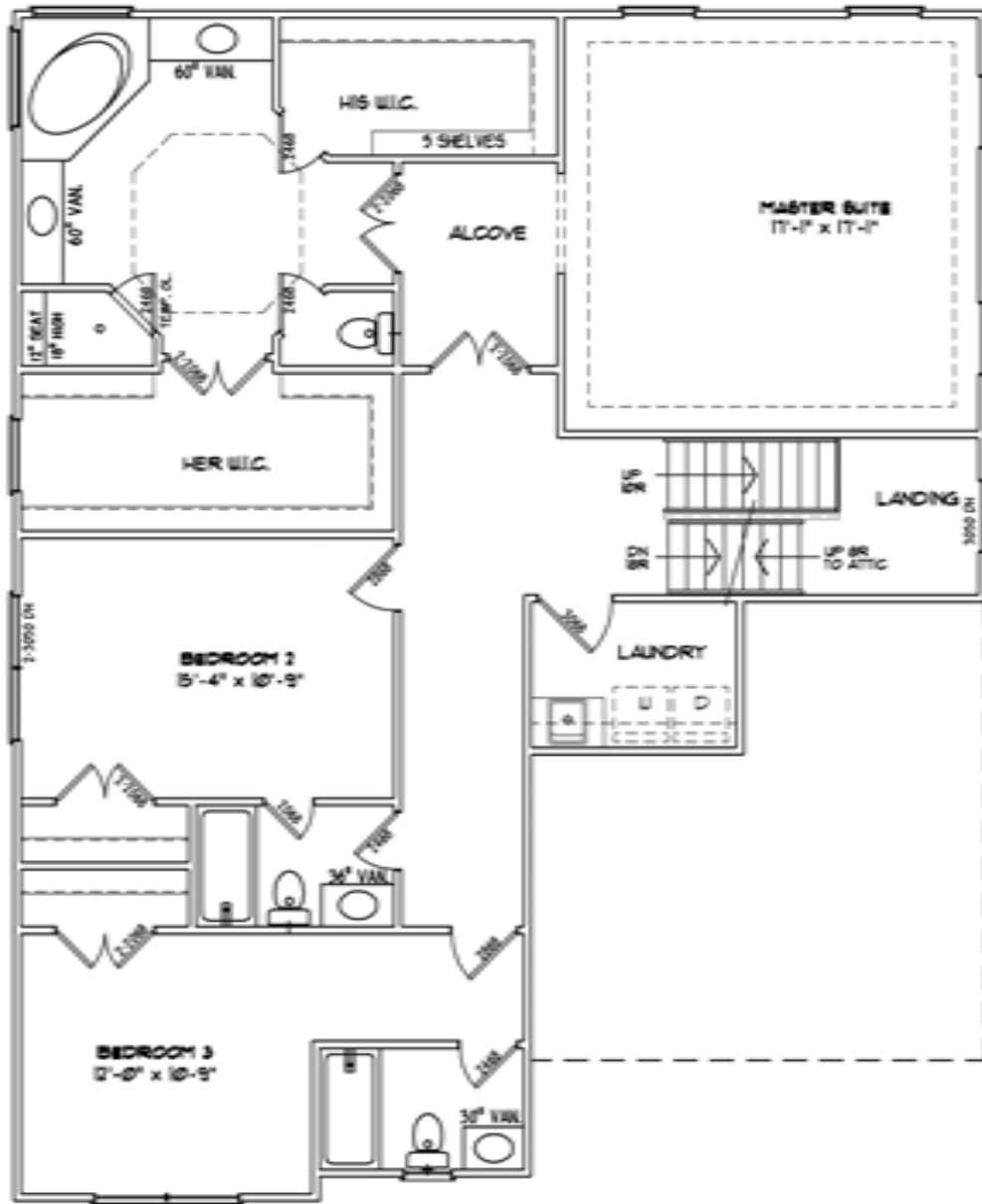
ALEXANDRIA III UPPER LEVEL
